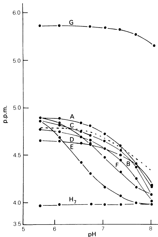
Figure 2 The ^1\text{H} chemical shifts of the seven histidine C2 protons (A to G) plotted as a function of pH in the 1:1 complex of dihydrofolate reductase with the methotrexate \alpha -amide (II). The dotted line is the pH titration curve for His F (His 28) in the complex of dihydrofolate reductase with methotrexate.
